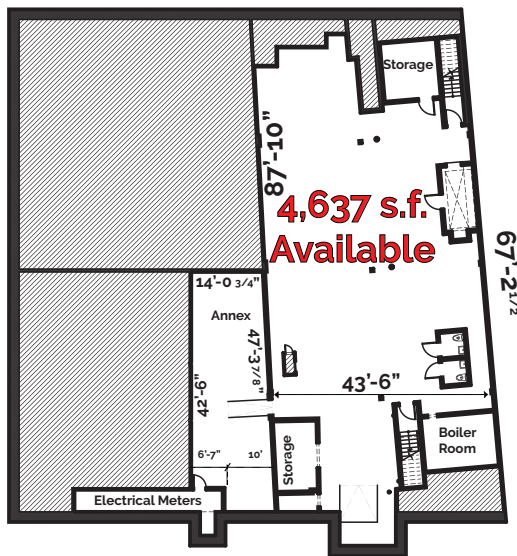
Existing Cellar Partition Plan
